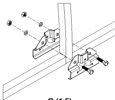
G (1:5)
